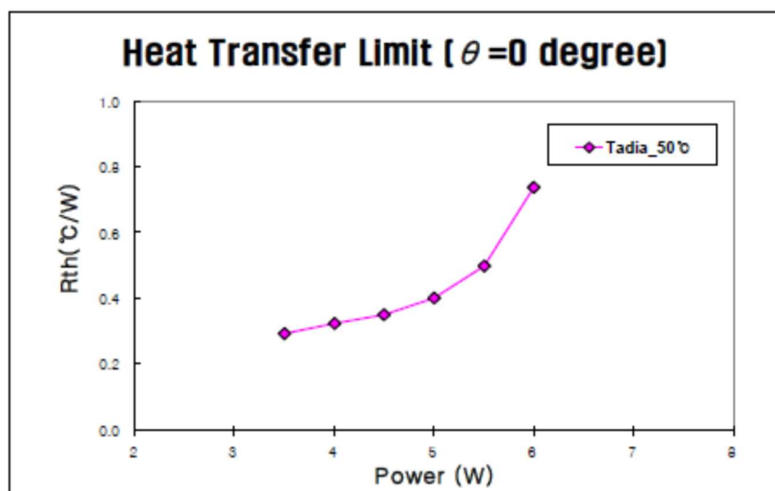
Fig. 3 Maximum Heat Transfer Rate at \theta=0^\circ , T_{adia}=50^\circ\text{C} ( L_e=28\text{mm} , L_a=30\text{mm} , L_c=67\text{mm} )
