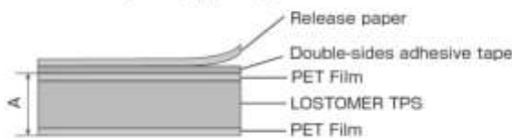
Adhesive tape equipped type / ALS20AF2-TC
